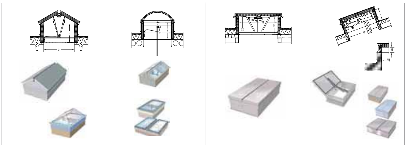
Orivent 51/ - Glass
